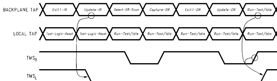
FIGURE 11. Local Scan Port Synchronization on Second Pass
