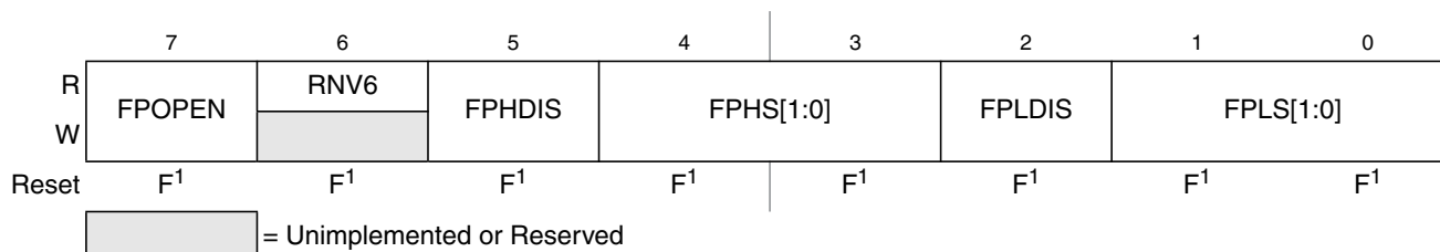
Figure 17-12. Flash Protection Register (FPROT)
