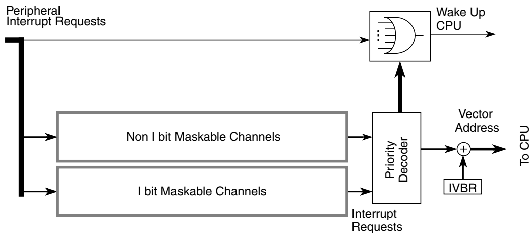
Figure 7-1. INT Block Diagram
