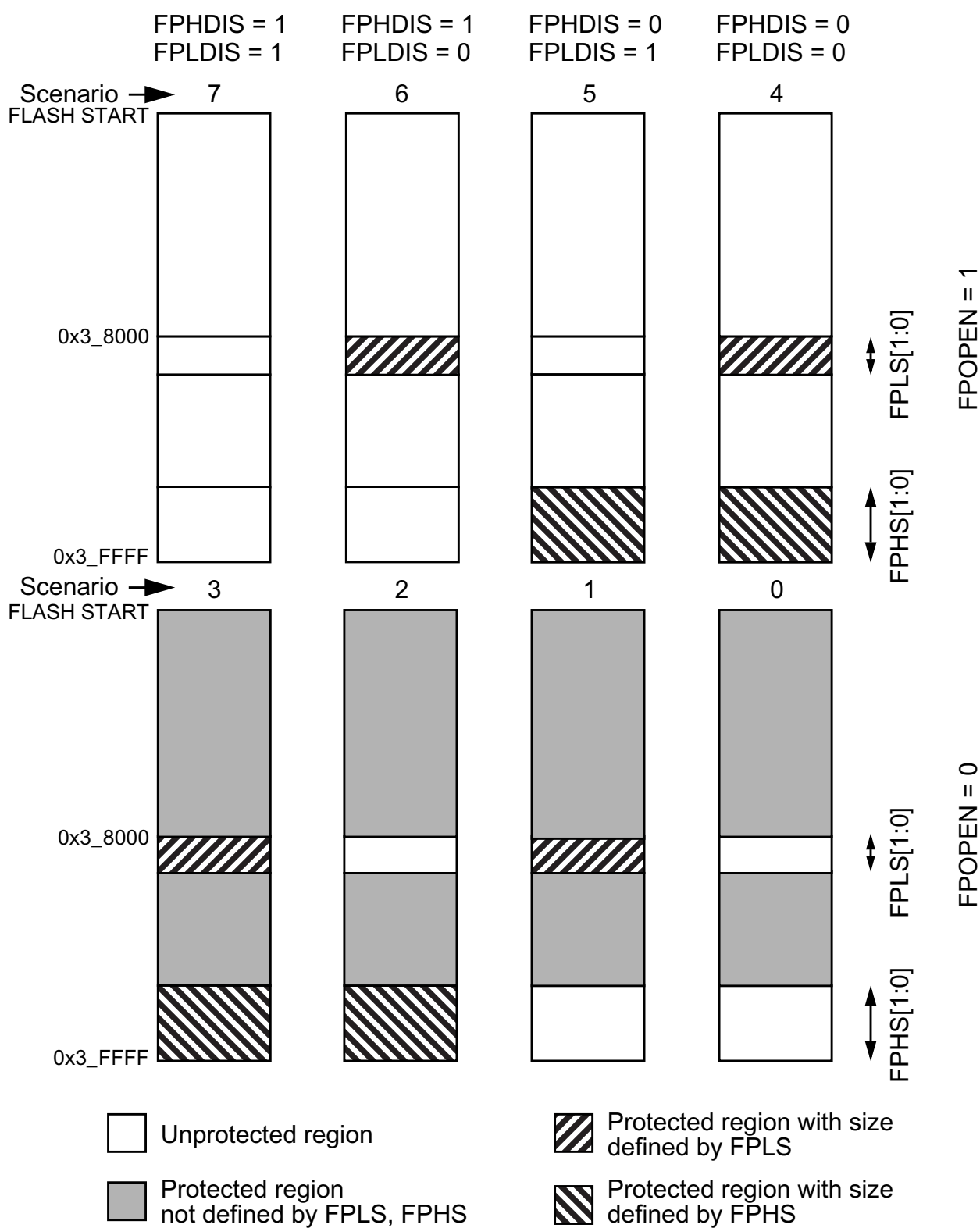
Figure 17-13. P-Flash Protection Scenarios
