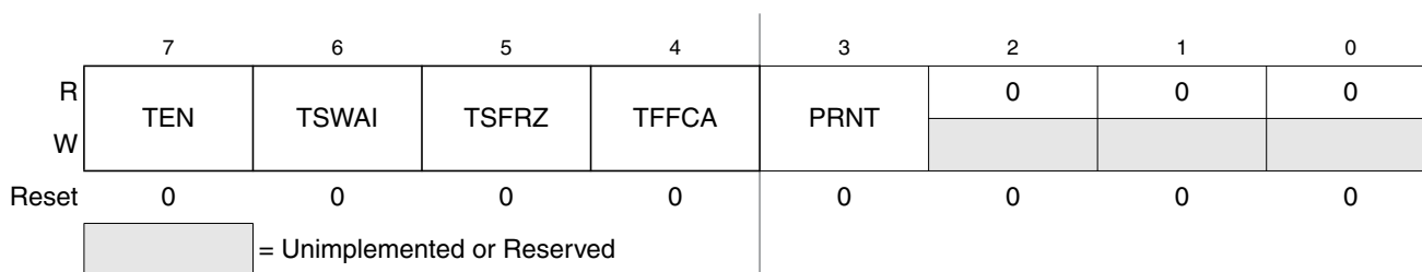
Figure 12-8. Timer System Control Register 1 (TSCR1)
