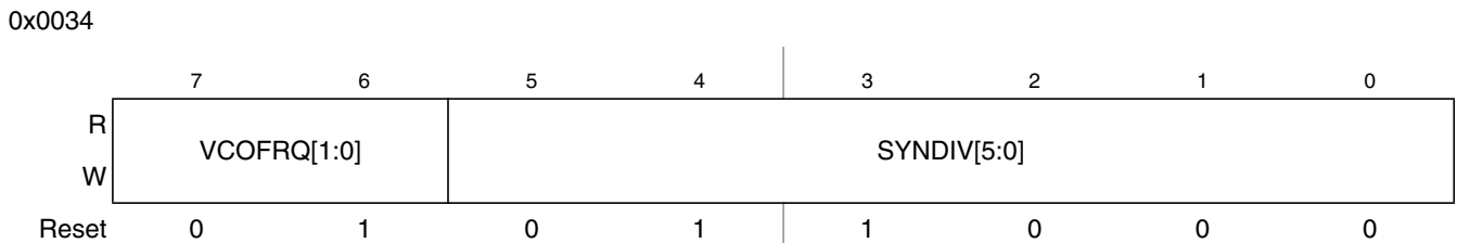
Figure 4-4. S12CPMU_UHV Synthesizer Register (CPMUSYNR)
