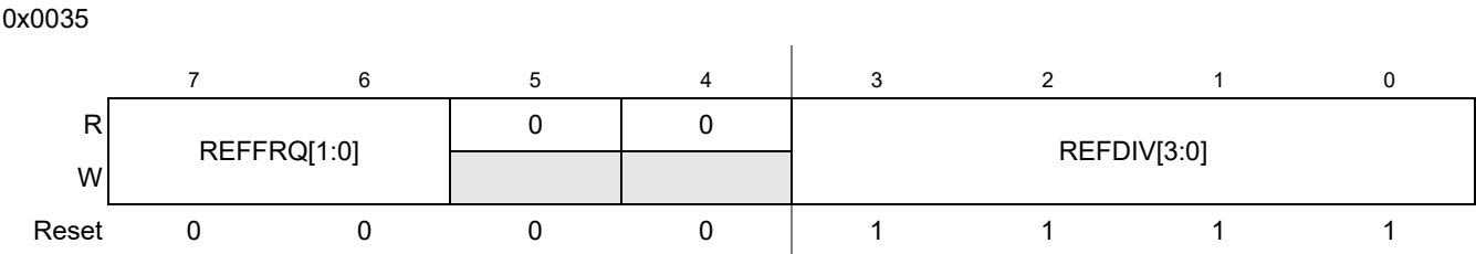
Figure 10-5. S12CPMU Reference Divider Register (CPMUREFDIV)
