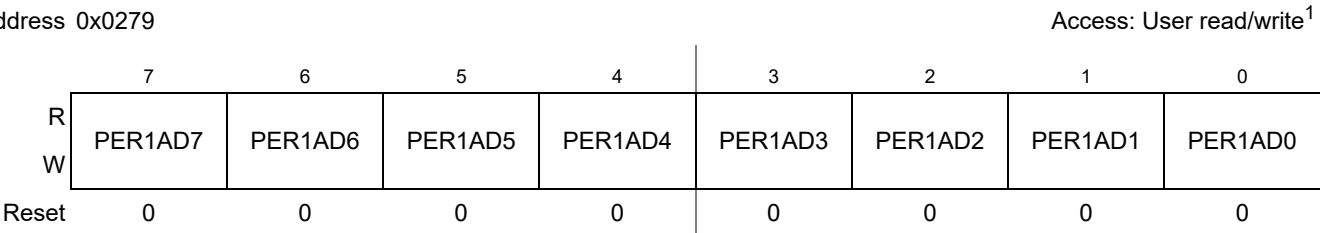
Figure 2-57. Port AD Pullup Enable Register (PER1AD)
