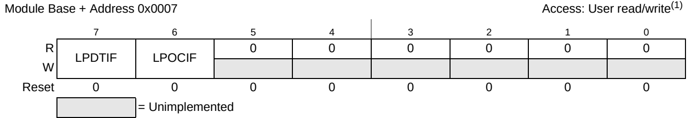
Figure 20-10. LIN Interrupt Flags Register (LPIF)
