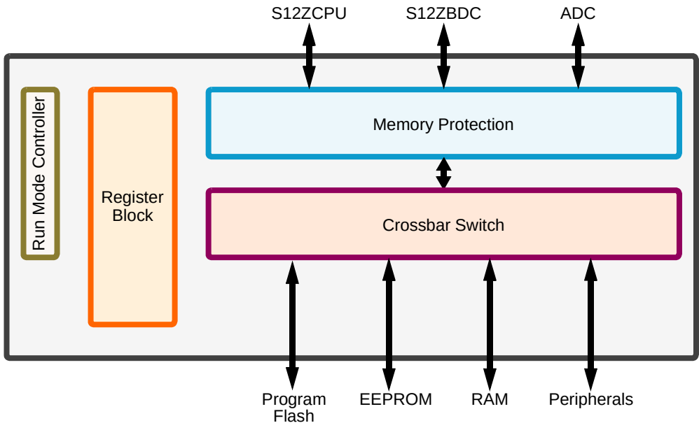
Figure 3-1. S12ZMMC Block Diagram
