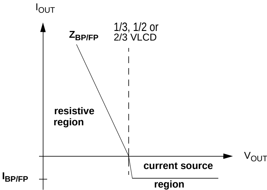
Figure E-3. buffer output characteristic
