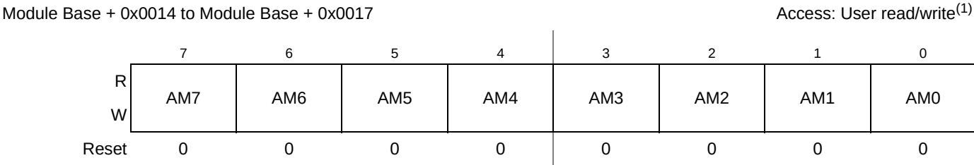
Figure 11-22. MSCAN Identifier Mask Registers (First Bank) — CANIDMR0–CANIDMR3
