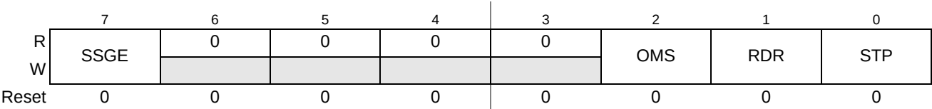
Figure 17-3. SSG Control Register (SSGCR)
