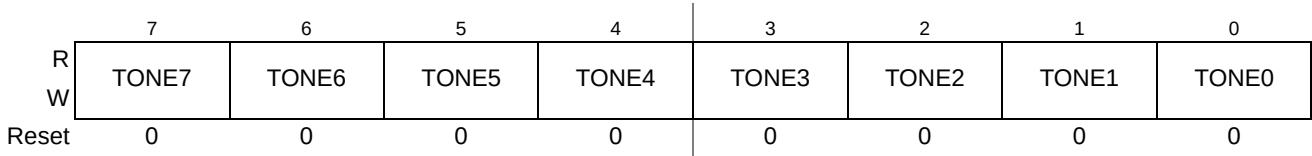
Figure 17-8. SSG Tone Register (SSGTONEL)
