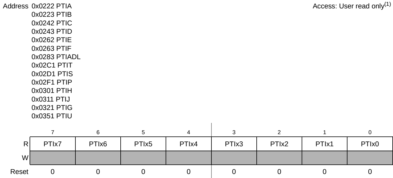
Figure 2-14. Port Input Register
