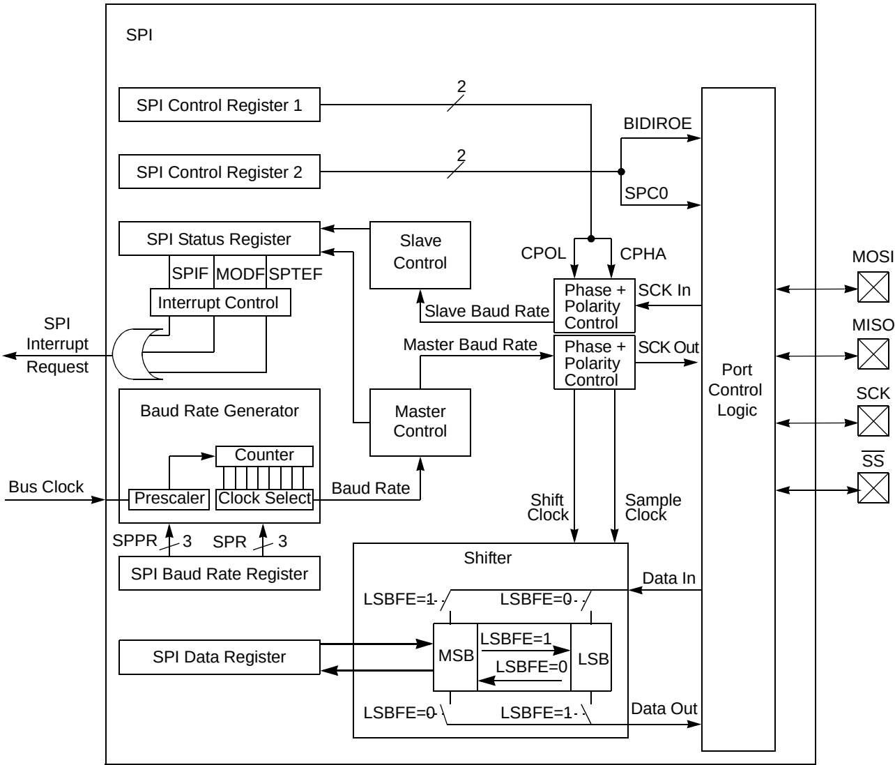
Figure 13-1. SPI Block Diagram
