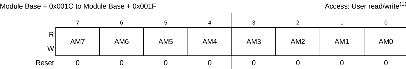
Figure 11-23. MSCAN Identifier Mask Registers (Second Bank) — CANIDMR4–CANIDMR7
