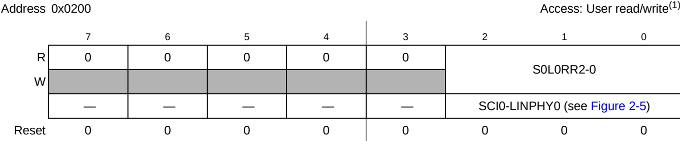
Figure 2-4. Module Routing Register 3 (MODRR3)
