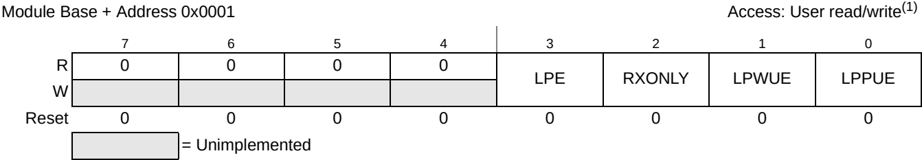
Figure 20-4. LIN Control Register (LPCR)
