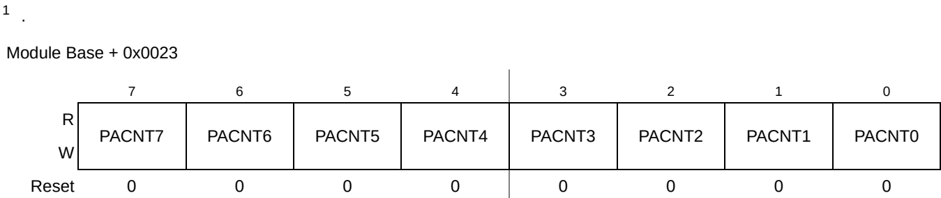
Figure 8-27. Pulse Accumulator Count Register Low (PACNTL)
