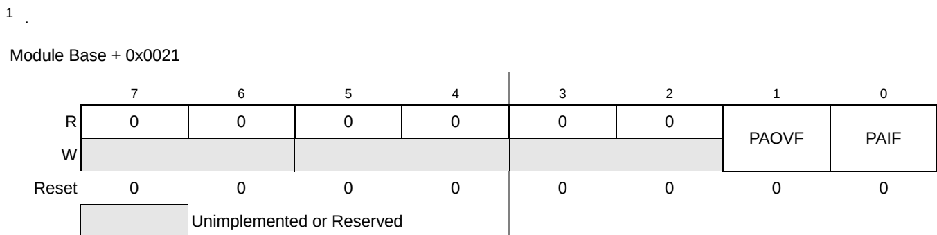
Figure 8-25. Pulse Accumulator Flag Register (PAFLG)
