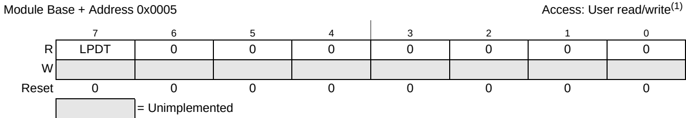
Figure 20-8. LIN Status Register (LPSR)
