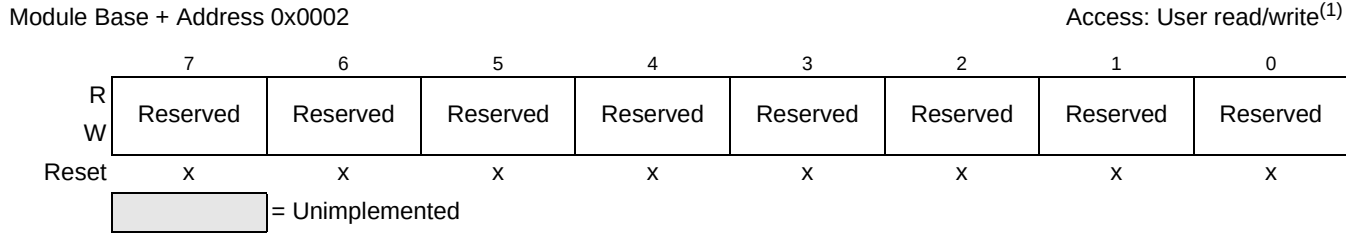
Figure 20-5. LIN Test register
