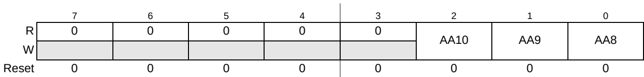
Figure 17-11. SSG Amplitude Adjustment (SSGAH)
