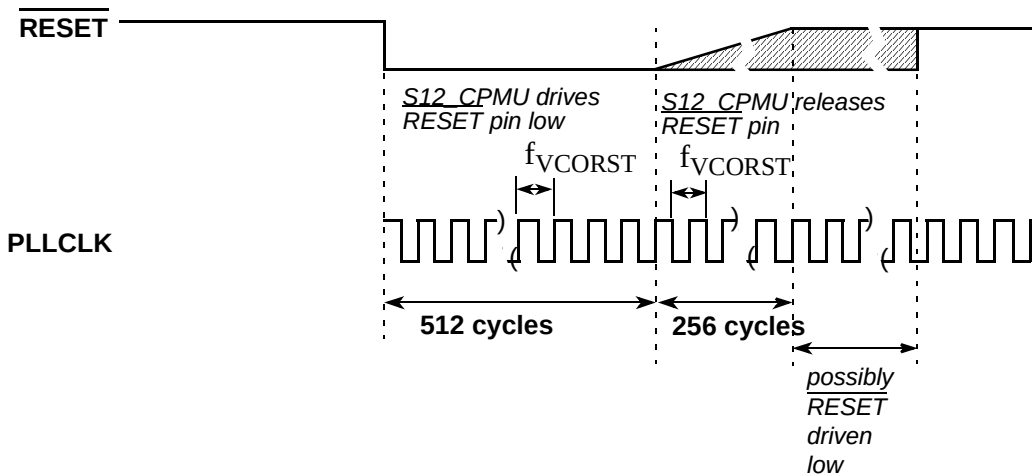
Figure 7-40. RESET Timing
