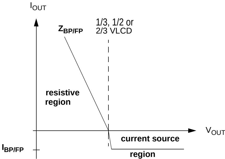
Figure E-3. buffer output characteristic
