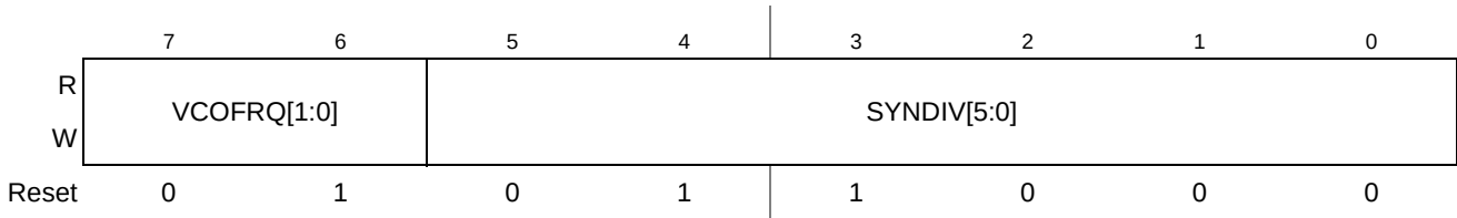
Figure 7-5. S12CPMU_UHV_V5 Synthesizer Register (CPMUSYNR)
