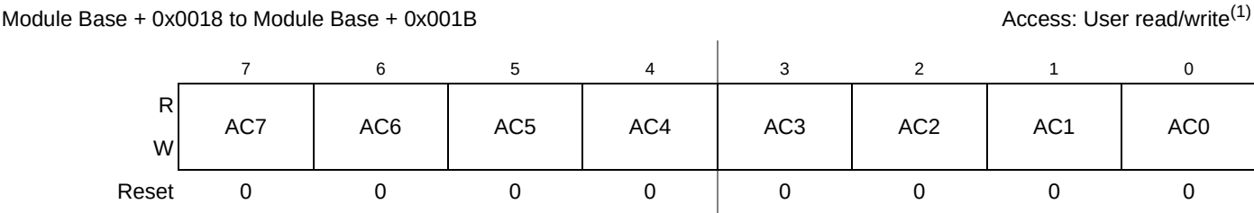
Figure 11-21. MSCAN Identifier Acceptance Registers (Second Bank) — CANIDAR4–CANIDAR7
