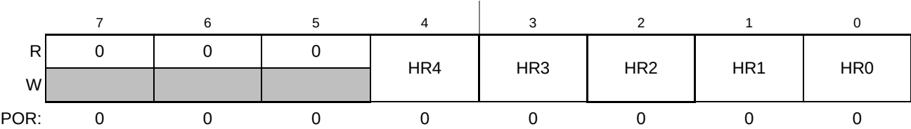
Figure 16-12. Hour Register (HRR)
