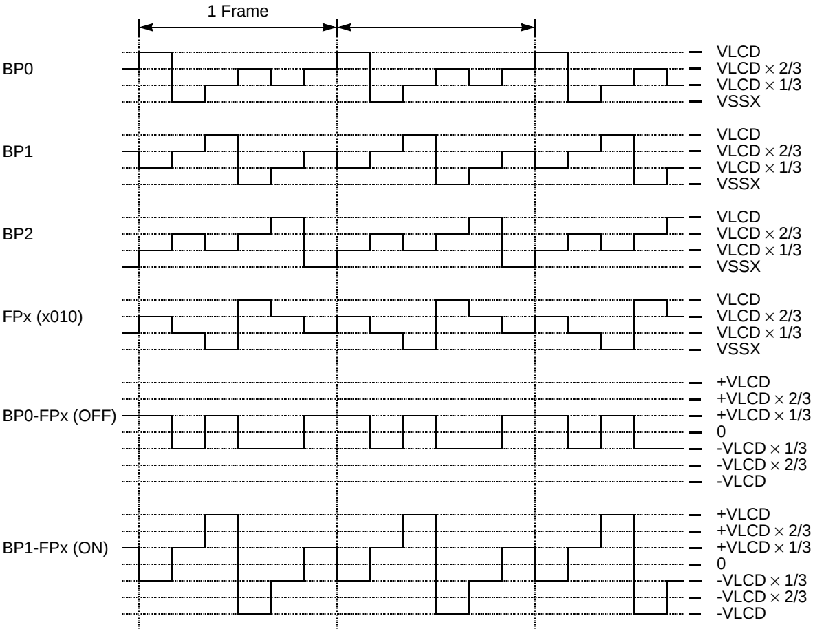
Figure 15-14. 1/3 Duty and 1/3 Bias
