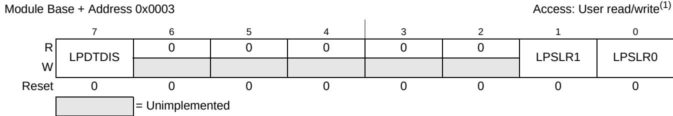
Figure 20-6. LIN Slew Rate Mode Register (LPSLRM)
