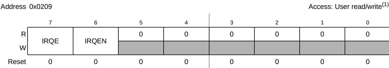
Figure 2-7. IRQ Control Register (IRQCR)
