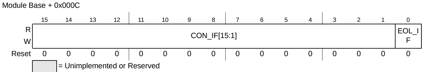
Figure 10-15. ADC Conversion Interrupt Flag Register (ADCCONIF)
