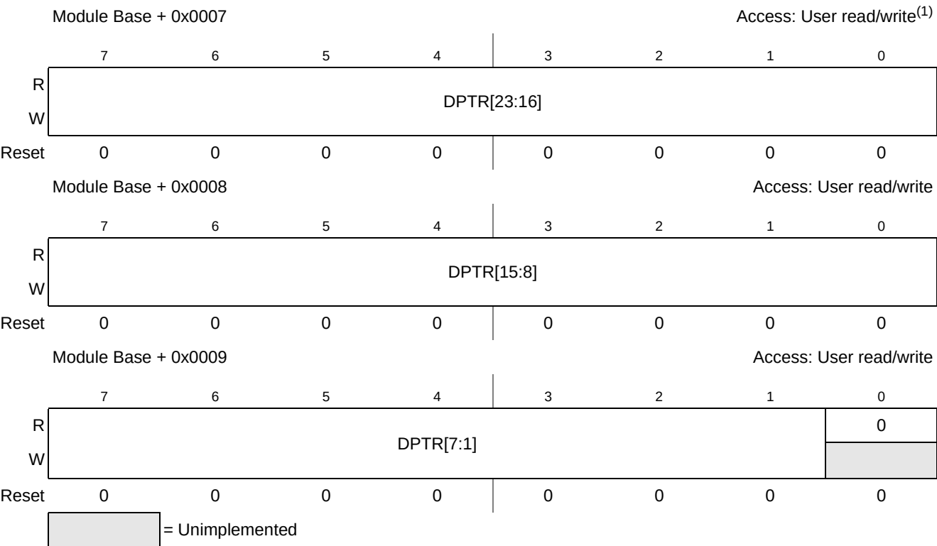
Figure 18-5. ECC Debug Pointer Register (ECCDPTRH, ECCDPTRM, ECCDPTRL)
