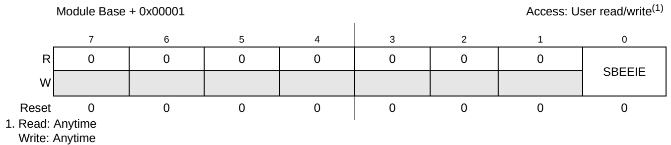
Figure 18-3. ECC Interrupt Enable Register (ECCIE)
