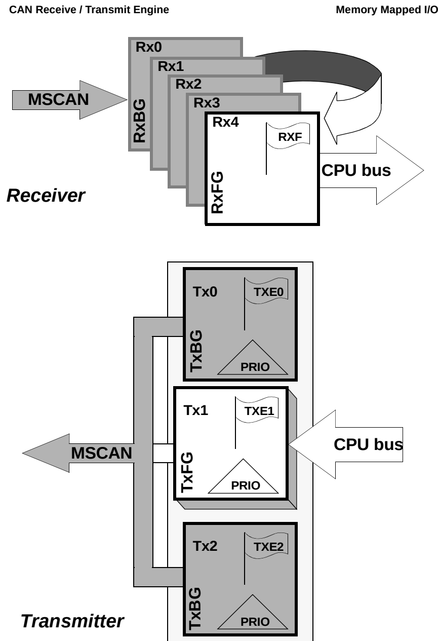
Figure 11-39. User Model for Message Buffer Organization
