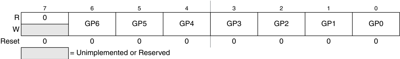
Figure 3-6. Global Page Index Register (GPAGE)
