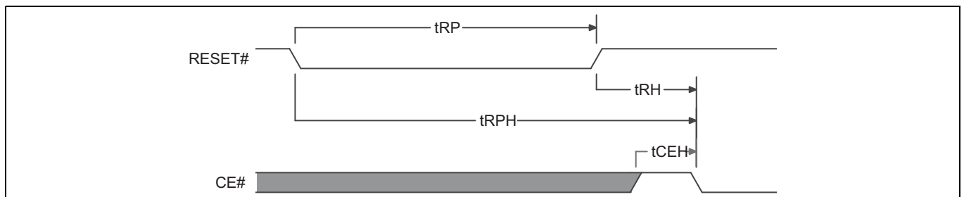
Figure 16 Hardware Reset
