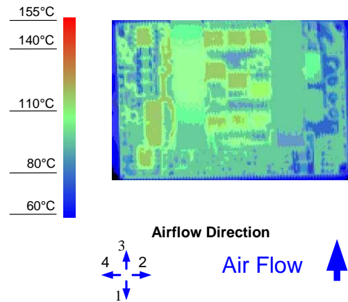
Figure 10. Thermal Image for Airflow Direction 3 (27A output, 55°C ambient, 200 LFM, typical Vin, open frame, soldered interface)
