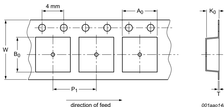
Fig 22. Carrier tape dimensions
