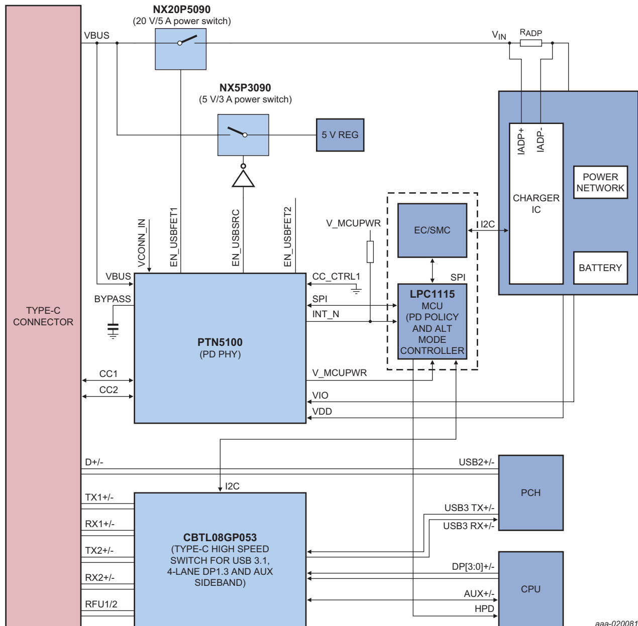
Fig 8. Illustrative diagram of Notebook/Ultrabook/Tablet application (Separate source and sink power paths): PD Provider/Consumer role (DFP role under Normal power/battery; UFP role under dead battery condition) 2 of 2
