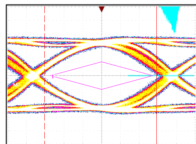
After ReDriver
