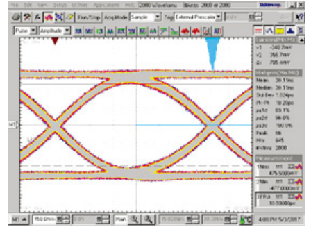
Trace=18-in, EQ=10.2dB
