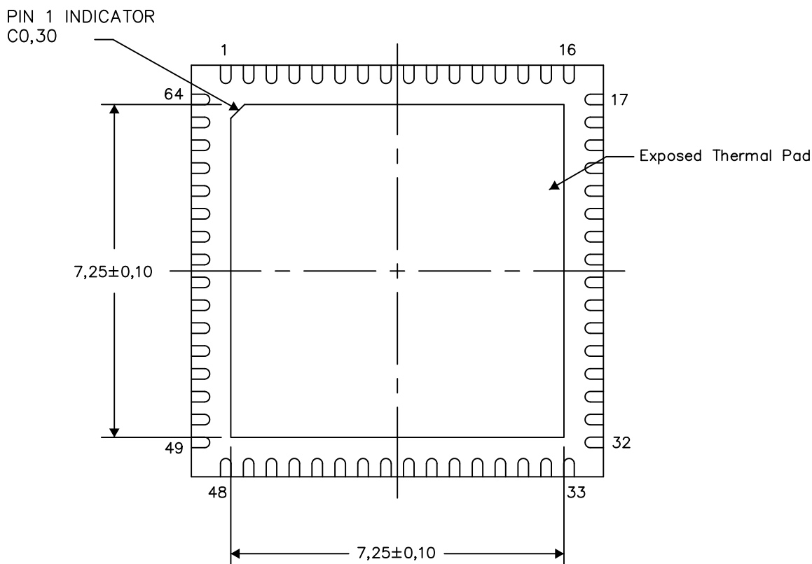
Bottom View
