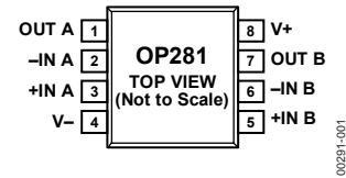
Figure 1. 8-Lead Narrow-Body SOIC (R Suffix)
