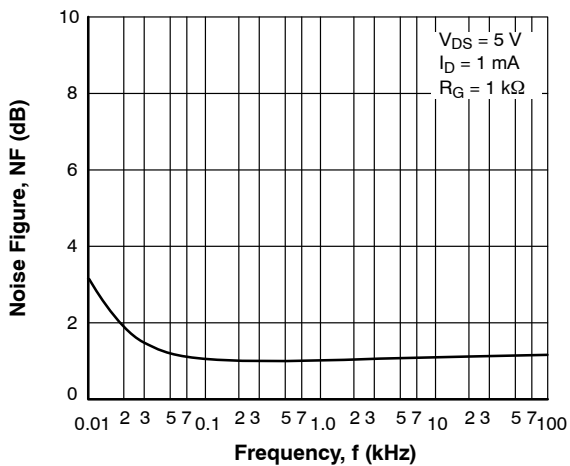
Figure 10. NF - f
