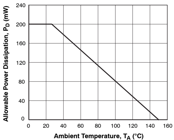
Figure 12. P_D - T_A
