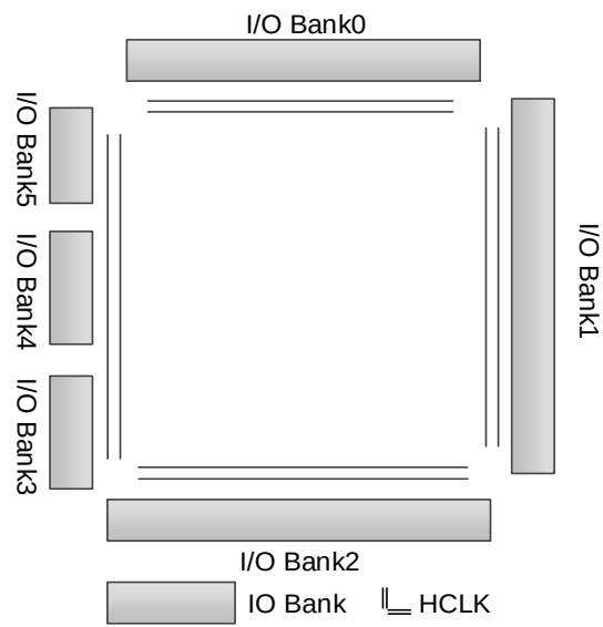
Figure 2-18 GW1NR-4 HCLK Distribution
