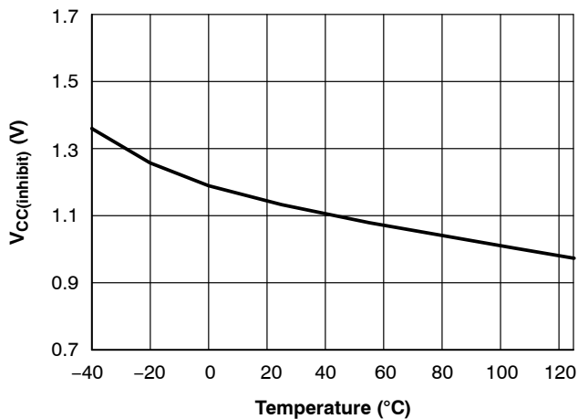
Figure 7. V_{CC(inhibit)} vs. Junction Temperature
