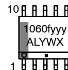
SOIC-10 CASE 751BQ AD or BD SUFFIX
