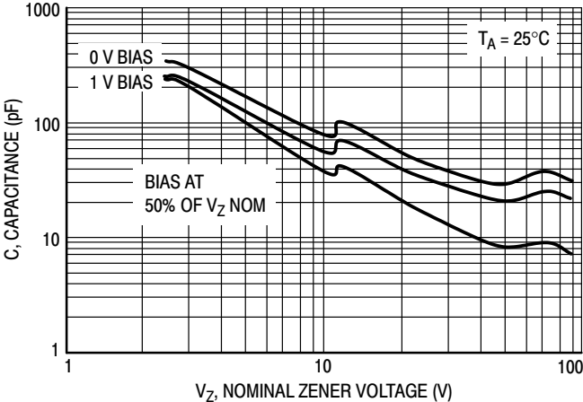
Figure 6. Typical Capacitance
