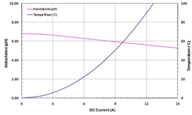
MMD-10DZ-6R8M-V1-RU
