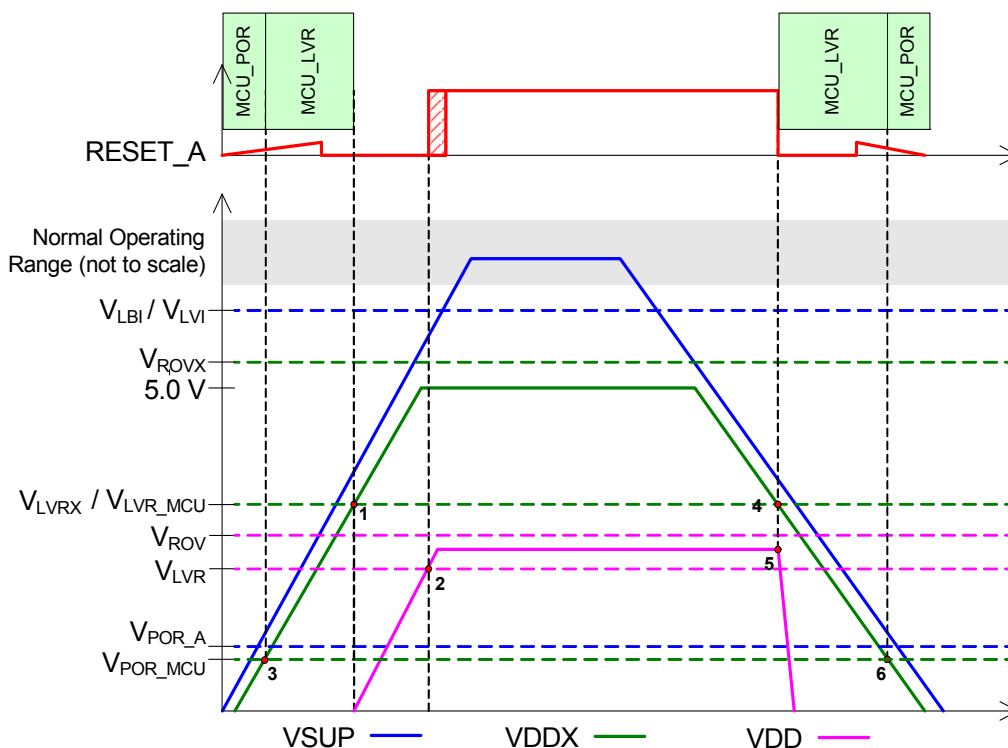
Figure 18. Power Up / Down Sequence
