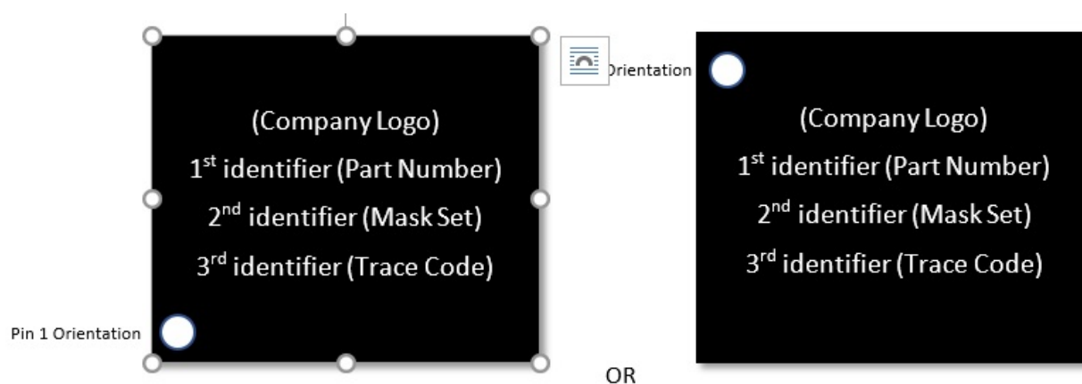
Figure 26. Package Marking
