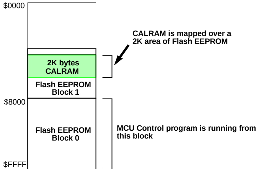
Figure 34 Map CALRAM over Flash EEPROM
