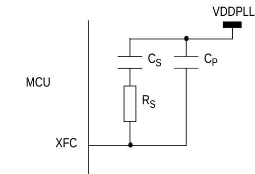
Figure 111 PLL Loop Filter Connections
