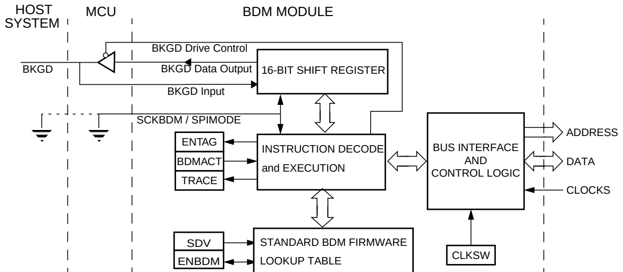
Figure 99 Block Diagram of BDM in Single Wire Mode
