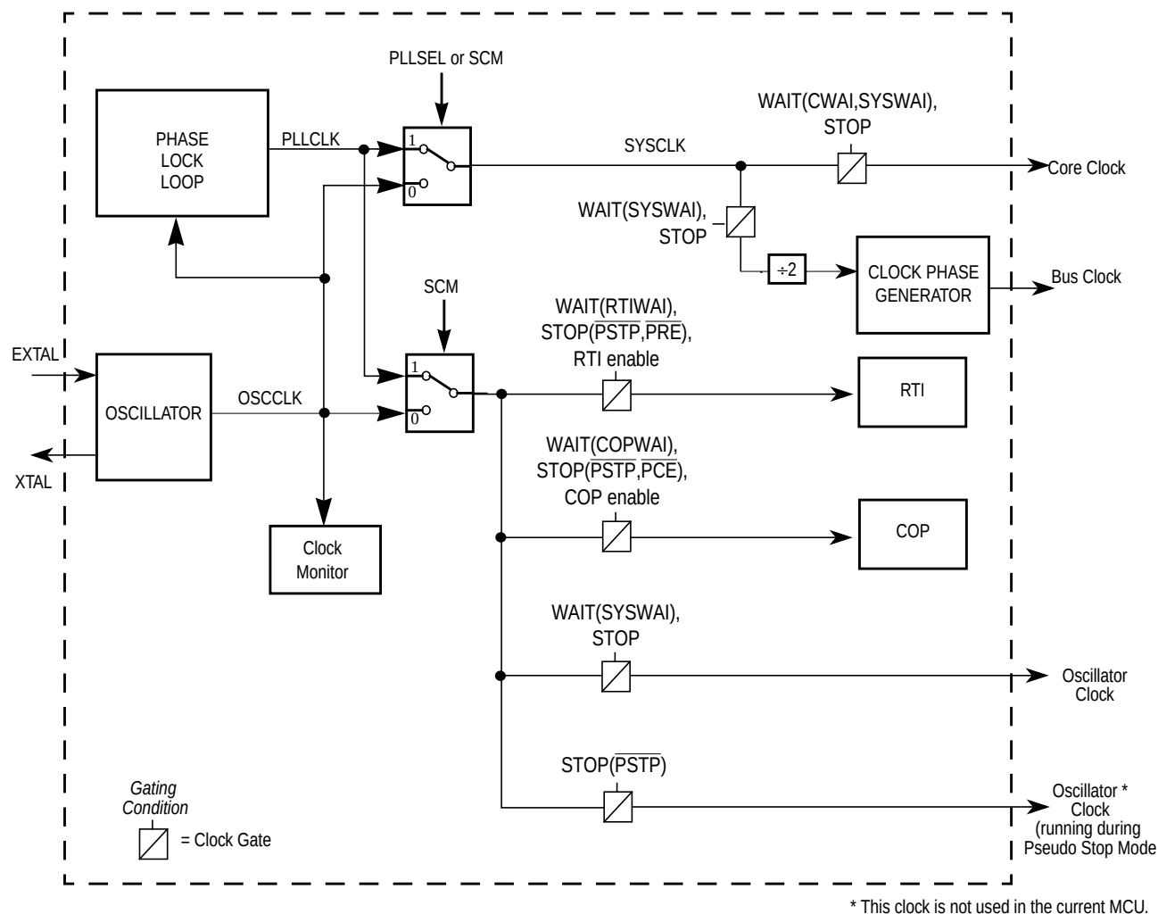
Figure 47 Clock Generator
