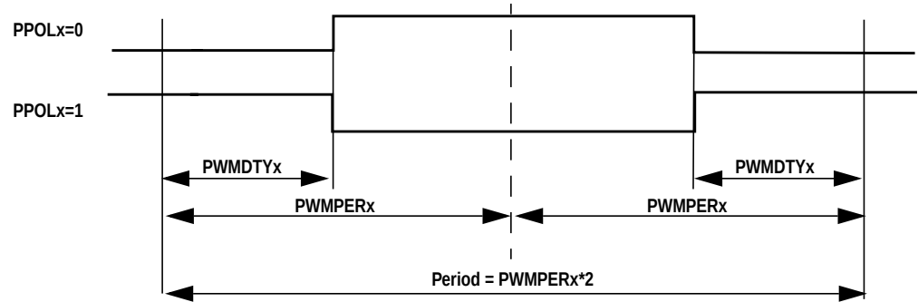
Figure 64 PWM Center Aligned Output Waveform
