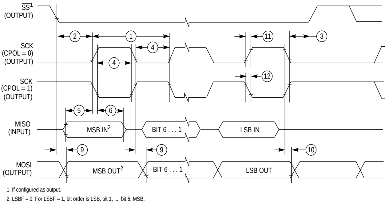
Figure 112 SPI Master Timing (CPHA = 0)
