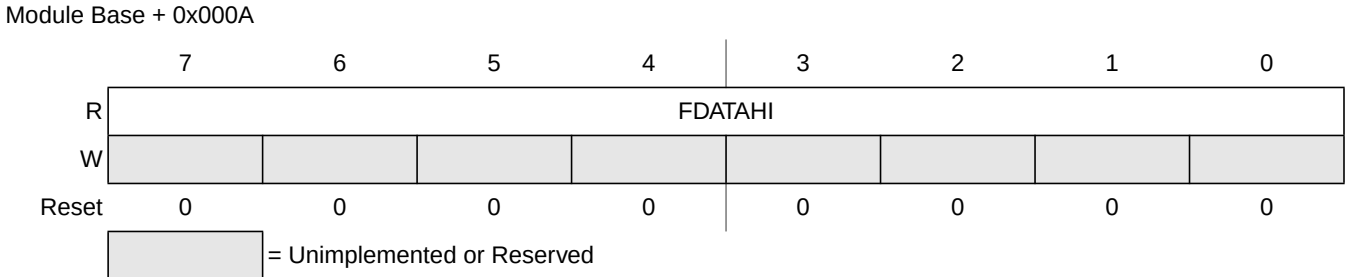
Figure 2-17. Flash Data High Register (FDATAHI)
