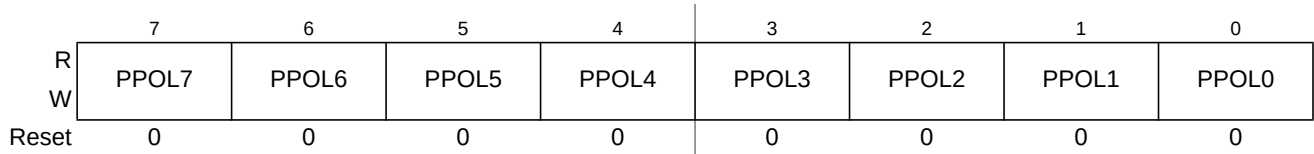
Figure 12-4. PWM Polarity Register (PWMPOL)
