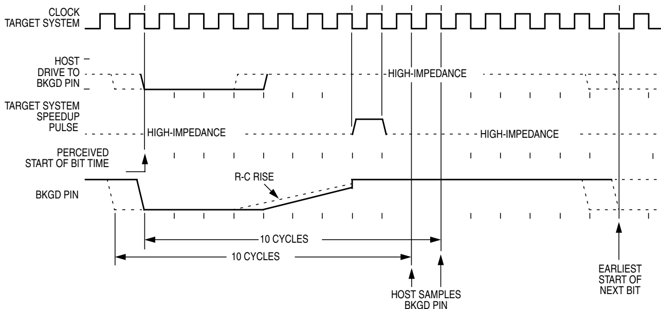
Figure 15-8. BDM Target-to-Host Serial Bit Timing (Logic 1)
