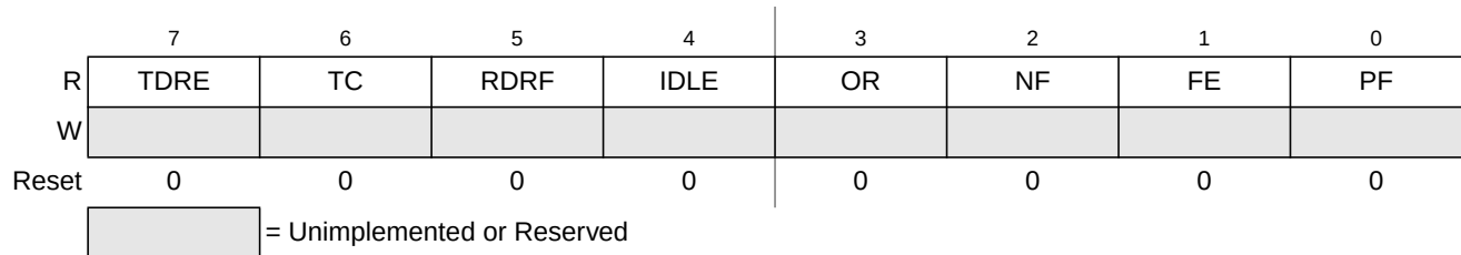
Figure 10-6. SCI Status Register 1 (SCISR1)
