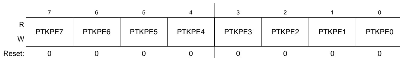
Figure 6-62. Internal Pull Enable for Port K Register (PTKPE)
