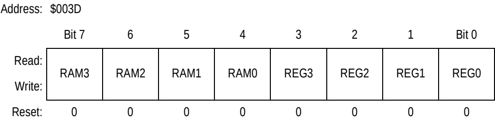
Figure 4-5. RAM and I/O Mapping Register (INIT)
