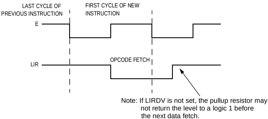
Figure 2-8. \overline{LIR} Timing
