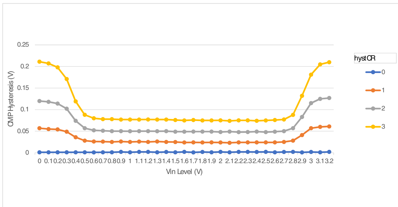
Figure 13. Typical hysteresis vs. Vin level ( V_{DD} = 3.3\text{ V} , PMODE = 0 )
