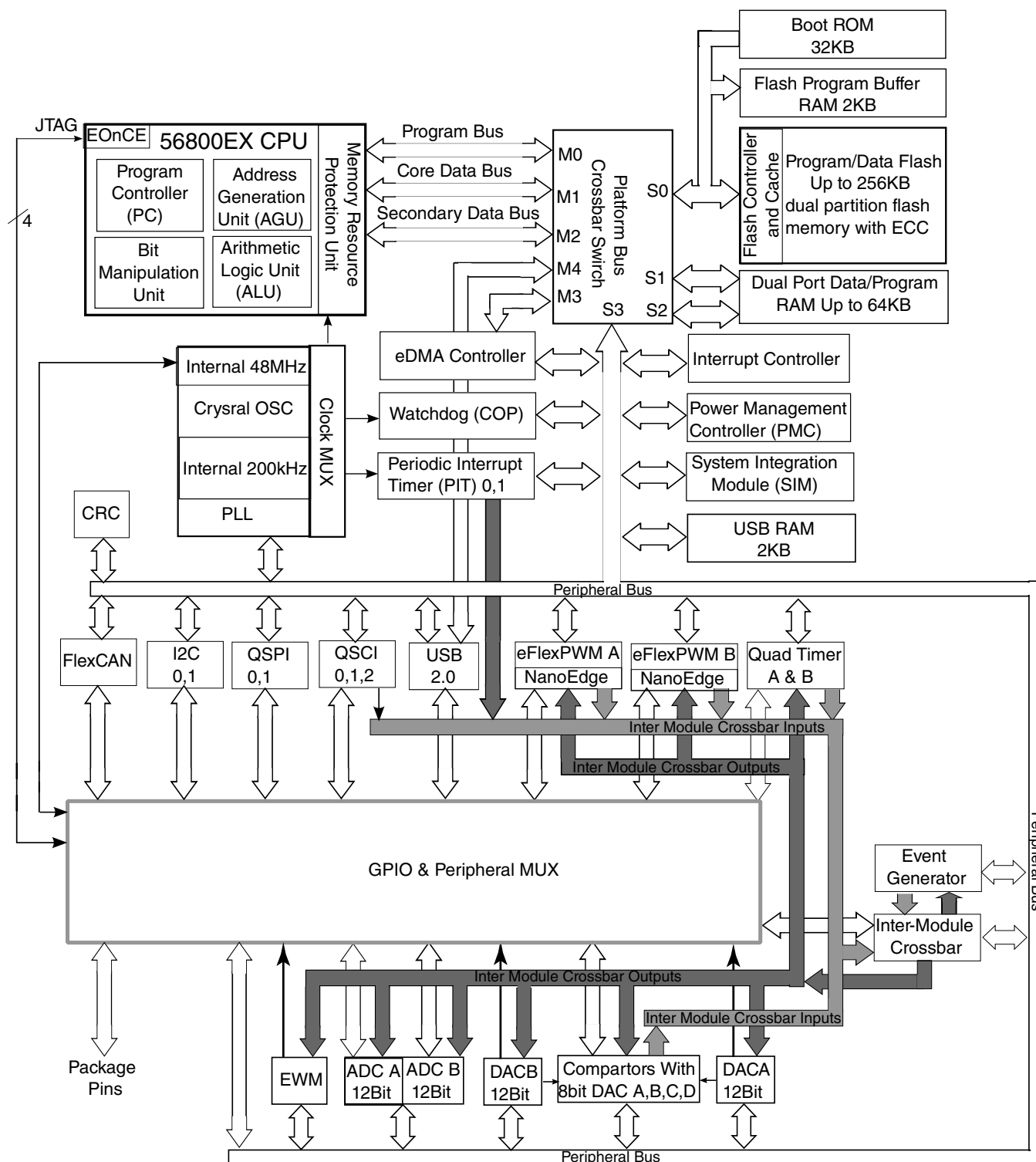
Figure 2. System diagram
