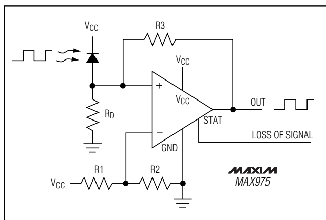
Figure 4. IR Receiver
