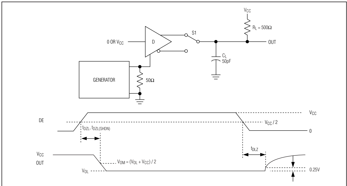
Figure 5. Driver Enable and Disable Times ( t_{DLZ} , t_{DLZ(SHDN)} )
