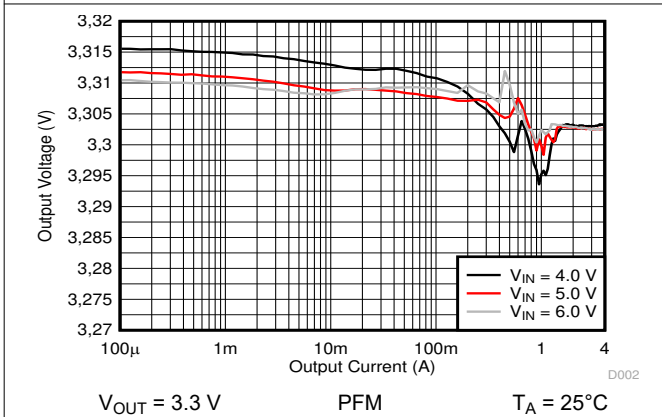
Figure 10-12. Output Voltage versus Output Current
