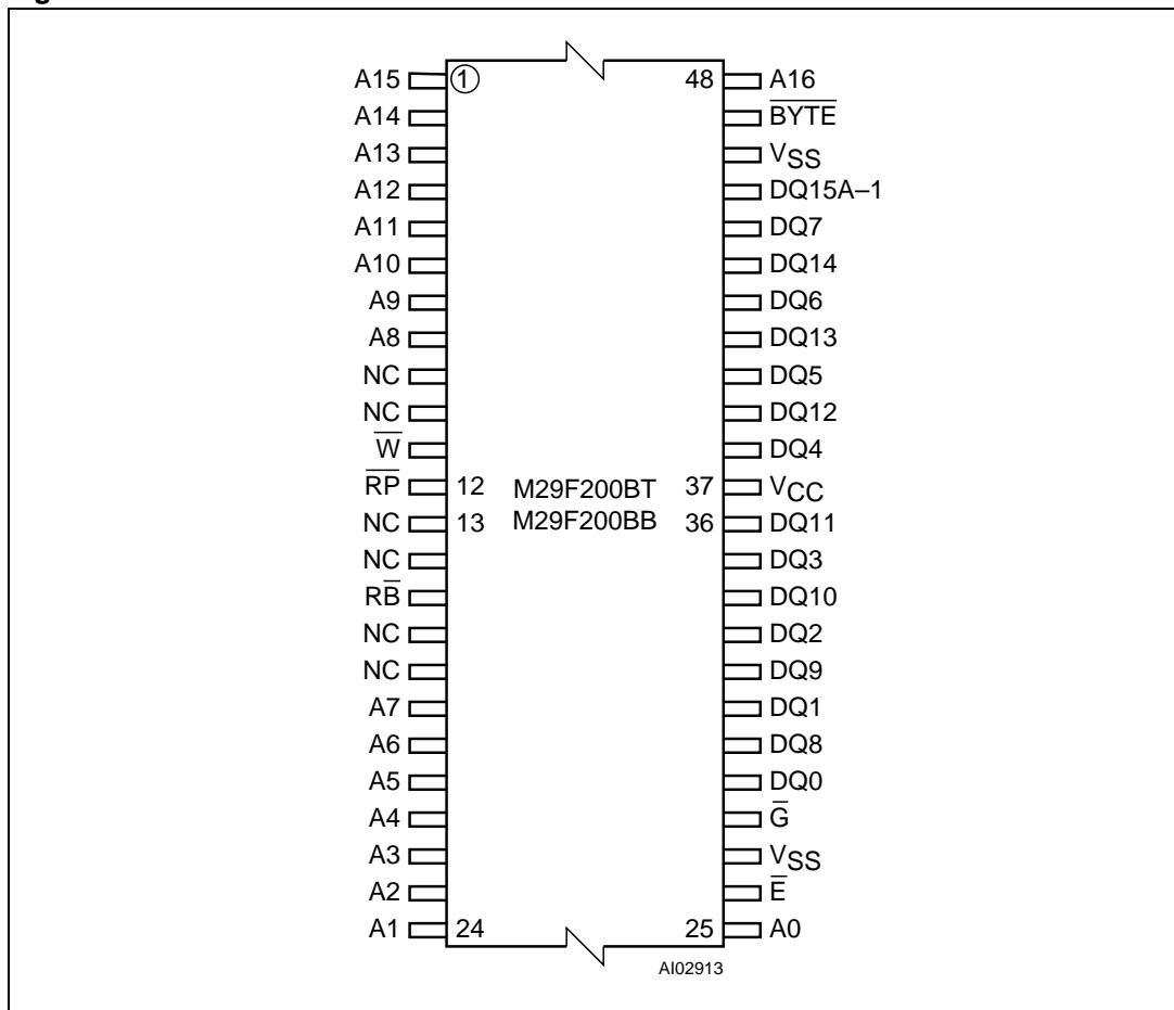
Figure 3. TSOP connections
