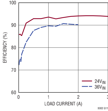
Efficiency, V_{OUT} = 15\text{V} , BIAS = 5V
