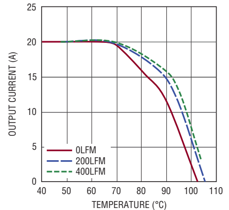
Figure 12. 12V IN to 1.0V OUT No Heat Sink
