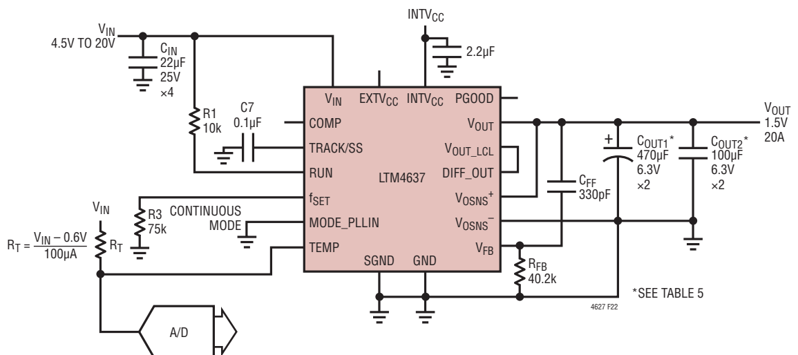
Figure 22. 4.5V to 20VIN, 1.5V at 20A Design
