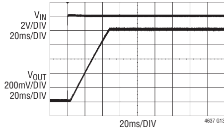
Turn-On No Load
