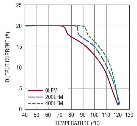
Figure 17. 5V IN to 2.5V OUT with Heat Sink
