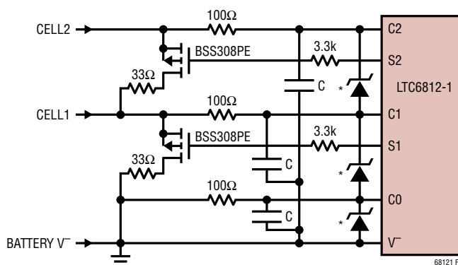
(b) Grounded Capacitor Filter
