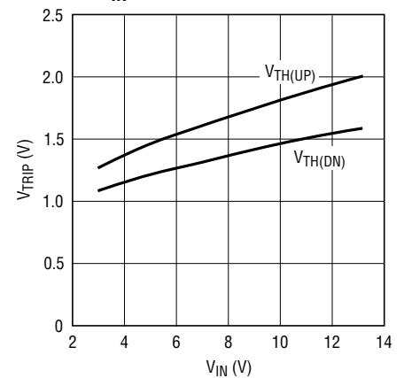
\overline{SHDN} Input Voltage Thresholds vs V_{IN}
