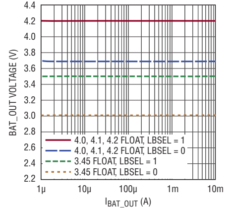
Battery Connect Voltage at BAT_OUT vs I_{\text{BAT\_OUT}}
