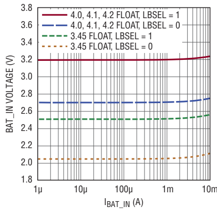
Battery Disconnect Voltage at BAT_IN vs I_{\text{BAT\_IN}}
