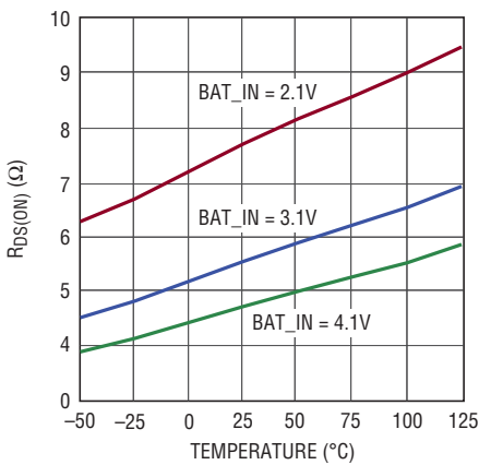
R_{\text{DS(ON)}} of Disconnect PMOS vs Temperature
