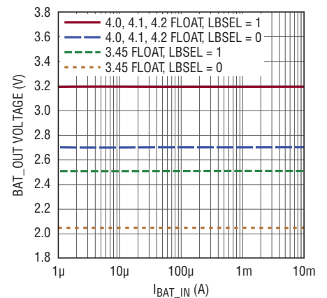
Battery Disconnect Voltage at BAT_OUT vs I_{\text{BAT\_IN}}
