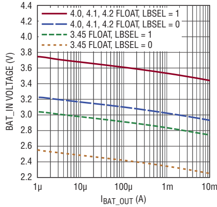
Battery Connect Voltage at BAT_IN vs I_{\text{BAT\_OUT}}
