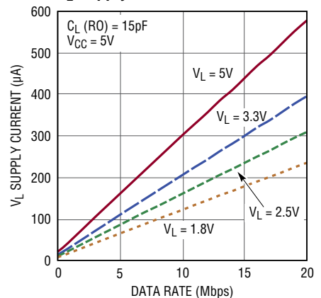
V_L Supply Current vs Data Rate
