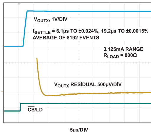
Figure 10. Settling 0 to 3.125 mA Step
