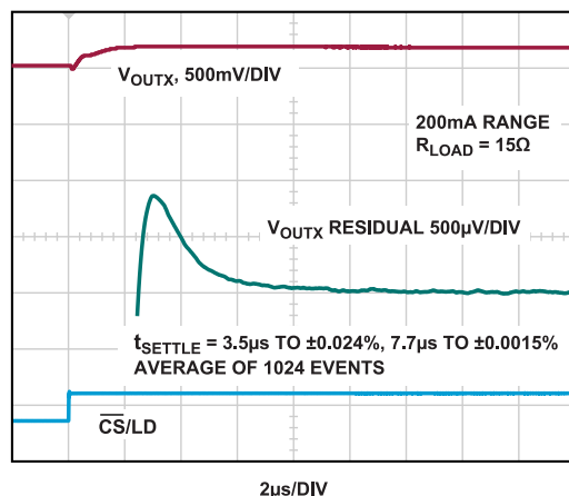
Figure 11. Settling 145 mA to 155 mA Step
