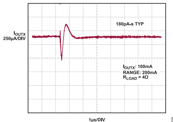
Figure 18. Mid-Scale Glitch
