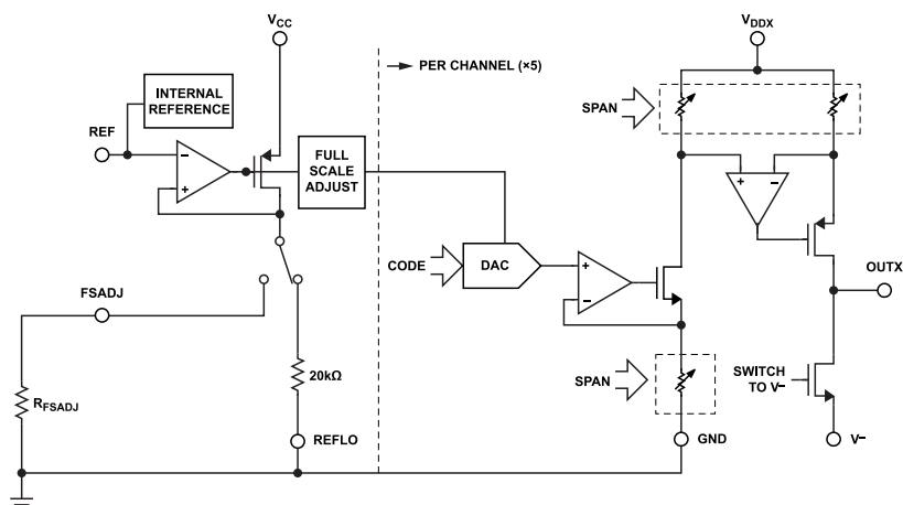
Figure 29. LTC2662 Single Channel Simplified Diagram
