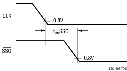
Voltage Waveform for t_{enSSO}
