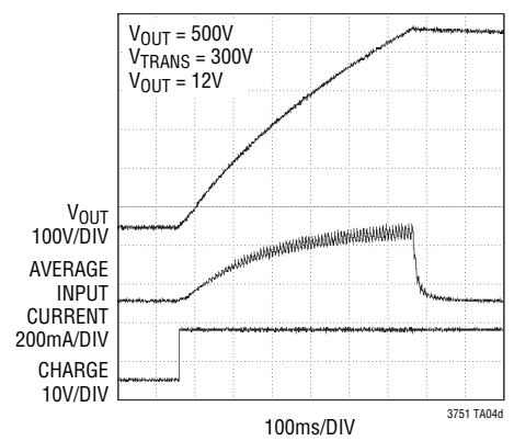
Charging Waveform
