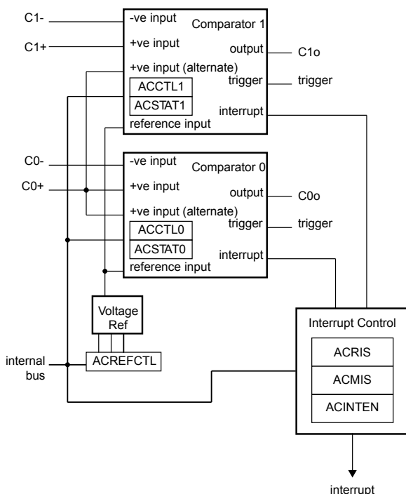
Figure 20-1. Analog Comparator Module Block Diagram
