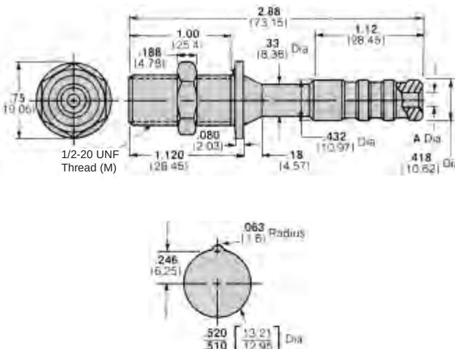
Recommended Panel Cutout for Bulkhead Mounting
