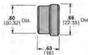
Plug Potting Shell Part Number 862544-1
