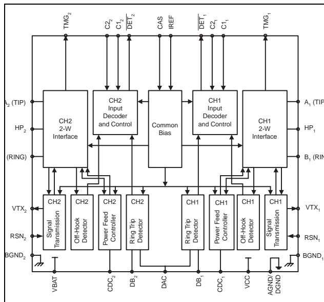
Figure 1 - Block Diagram
