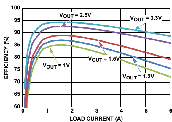
FIGURE 7. SINGLE CHANNEL, V_{IN} = 5\text{V}
