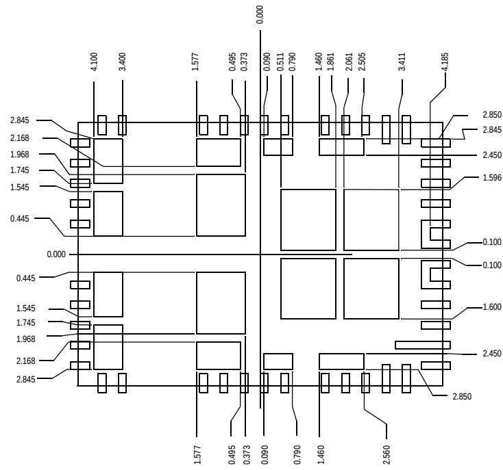
STENCIL PATTERN WITH 23 MOSLP TOP VIEW
