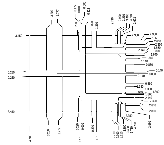
STENCIL PATTERN WITH 23 MOSLP TOP VIEW
