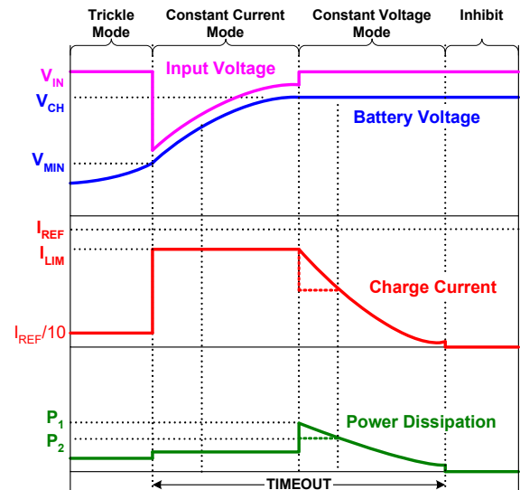
FIGURE 20. TYPICAL CHARGE CURVES USING A CURRENT-LIMITED ADAPTER
