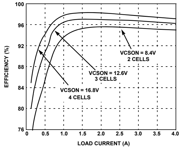
FIGURE 4. SYSTEM EFFICIENCY vs CHARGE CURRENT
