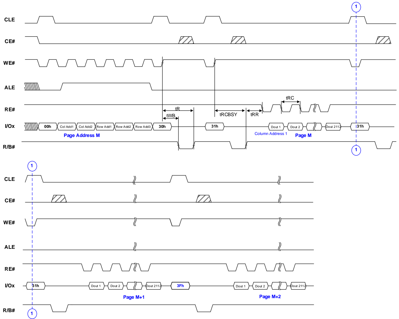
Figure 6.15.Cache Read Operation
