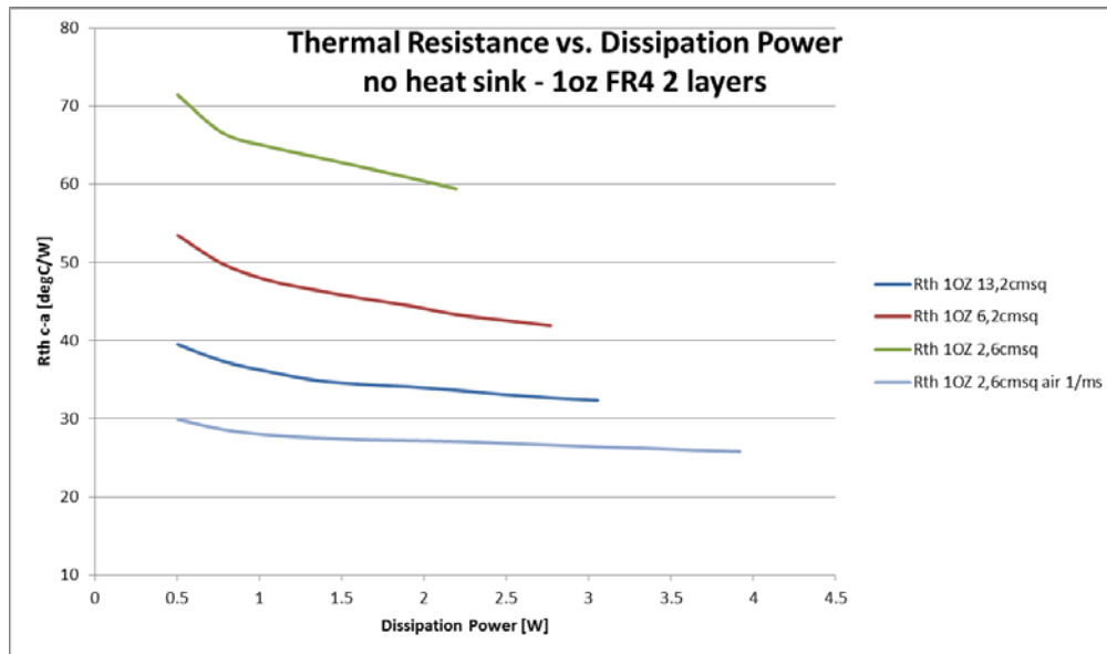
Figure 8 – Typical thermal resistance vs. power dissipation in the module (no heat sink) with 1oz FR4
