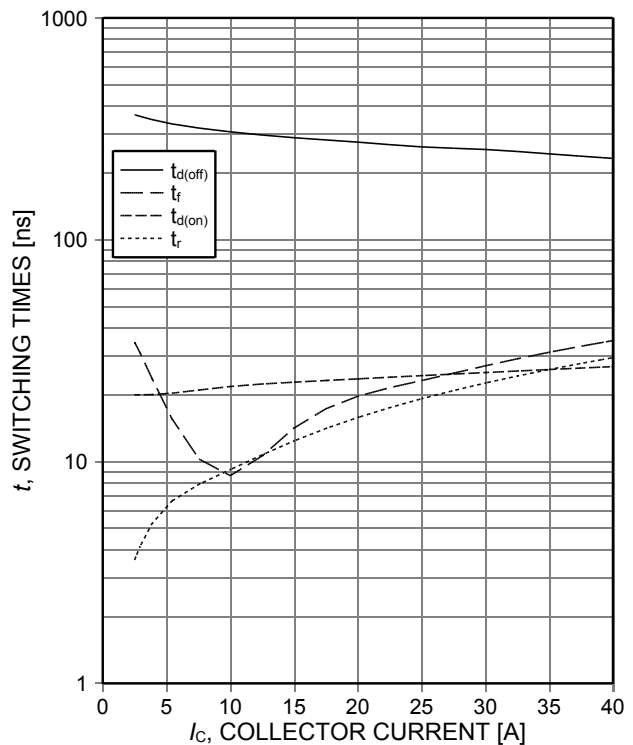
Figure 8. Typical switching times as a function of collector current (inductive load, T_{vj}=175^\circ\text{C} , V_{CE}=400\text{V} , V_{GE}=0/15\text{V} , R_{Gon}=23\Omega , R_{Goff}=23\Omega , dynamic test circuit in Figure E)
